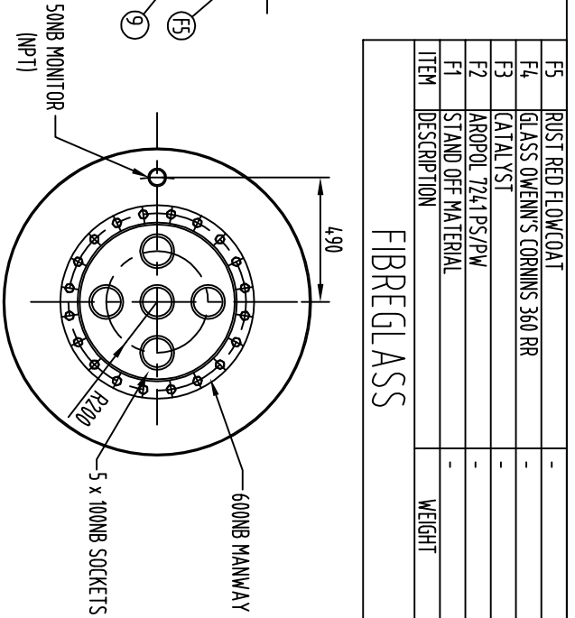
PLAN VIEW ON MANWAY
